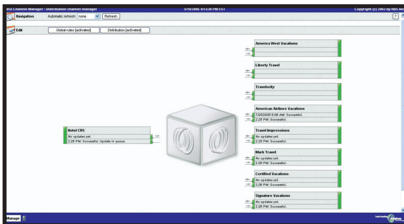
Figure 2: A channel management dashboard showing the real-time transaction activity between a hotel's CRS, PMS or RMS and its multiple distribution channels. Users can drill down to manage each link as needed. Courtesy of Hotel Booking Systems Incorporated.
